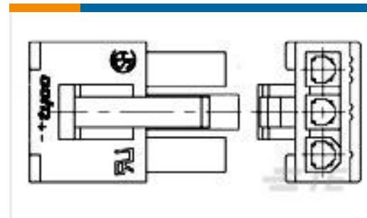
TE Part #1586027-5 5P SR RCPT VAL-U-LOK V0
