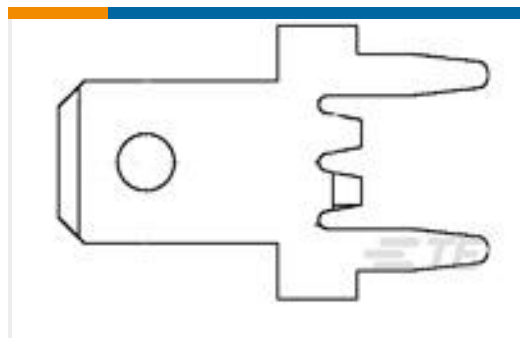
TE Part #63982-1 187 FASTON TAB TPBR
