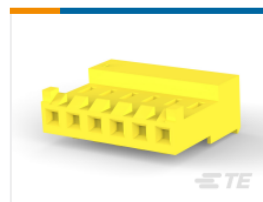
TE Part # 3-643818-6 06P MTA156 CONN ASSY 20AWG YEL
