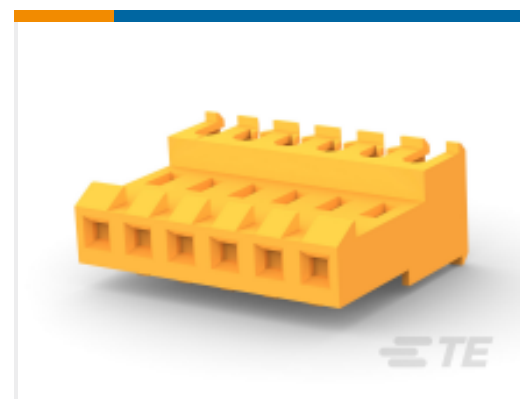
TE Part # 3-640599-6 06P MTA156 CONN ASSY 18AWG ORA
