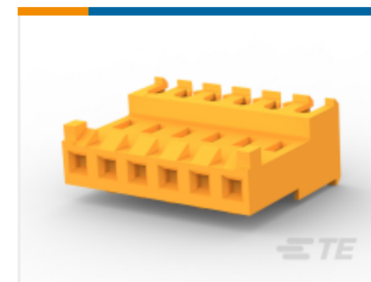
TE Part # 3-644465-6 06P MTA156 CONN ASSY 18AWG ORA
