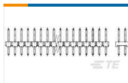
TE Part #1-2041051-4 AMPMODU 2.0mm PITCH, POST HDR
