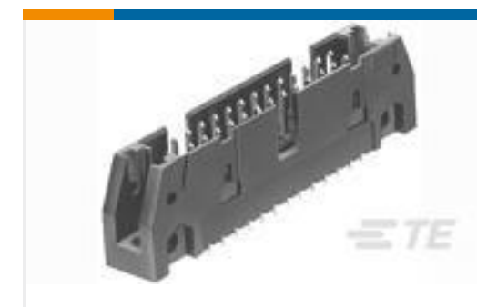
TE Part #102156-5 024 UNIV HDR SP 4S 30DP STD
