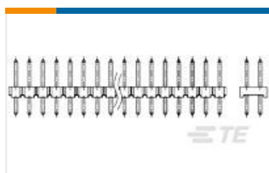
TE Part #2041051-1 AMPMODU 2.0mm PITCH, POST HDR
