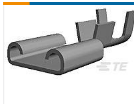
TE Part #42437-5 250 FASTON REC 14-10 AWG TPBZ
