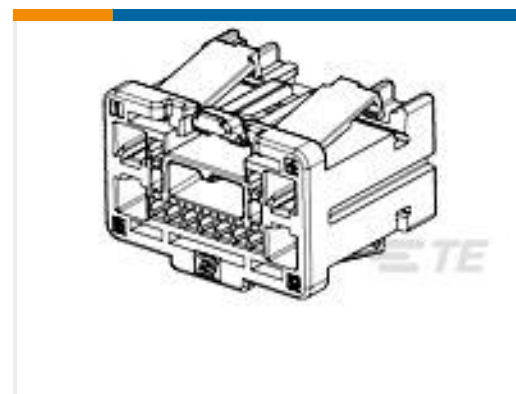
TE Part #1924667-1 13p Hybrid - 1pc Unsealed Plug, Key A
