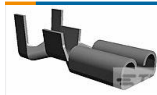
TE Part #62138-1 187 FASTON REC 24-20 TPBR
