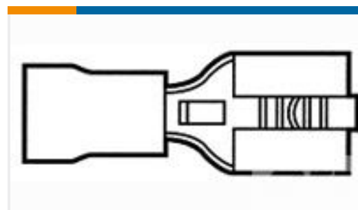
TE Part #55675-2 RECEPT,PIDG FASTON 22-18 250
