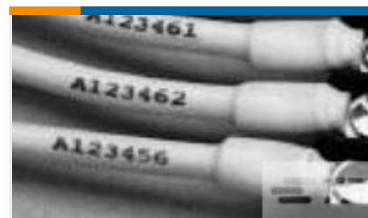
TE Part #5053082106 RNF-100-3/16-WH-STK
