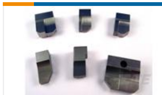
TE Part #1333203-4 ANVIL, COMBINATION .070
