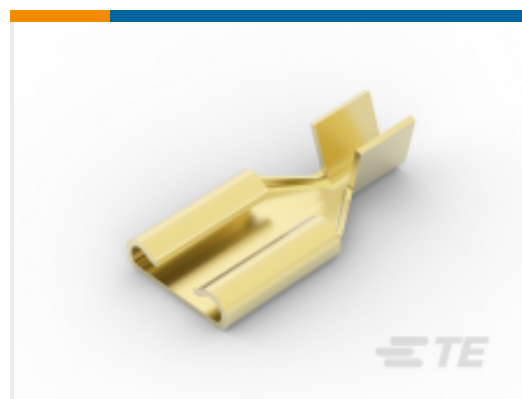
TE Part # 42845-1 250 FASTON REC 18-14 AWG BR
