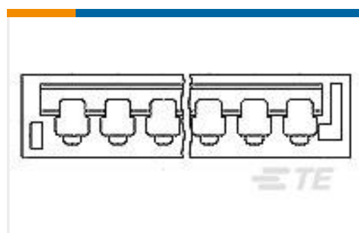
TE Part #640251-3 3.96mm Wire-to-board housing: receptacle, no mating alignment, SL 156
