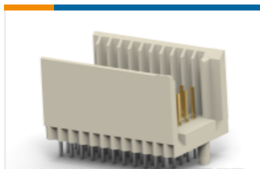
TE Part #5646529-1 Hard Metric Male Connector: Traditional Backplane, Mezzanine, 2mm
