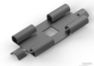
TE Part # 62751-1 FASTON 250 PCB TAB TPBR
