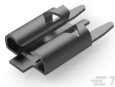
TE Part # 1217080-1 FASTON 205/250 PCB MOUNTED TPBR
