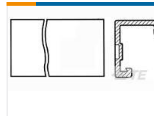
TE Part #640551-4 04P MTA156 COVER
