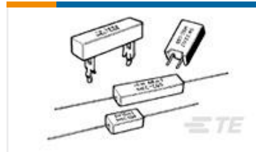
TE Part #1-1623783-3 SQM7 47K 2% (METAL FILM)
