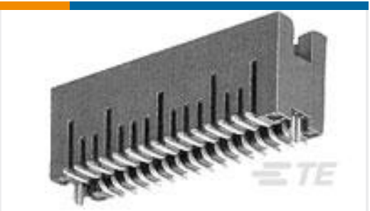
TE Part #5-104656-5 50 50/50 HDR DRST SFMNT .320 SN
