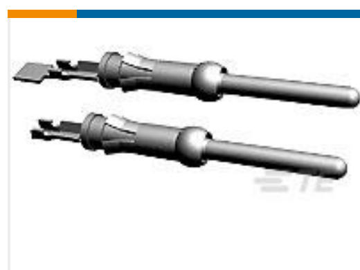
TE Part #66429-3 III+ PIN,30-26,15AU/FL,LP
