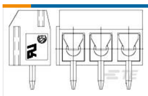
TE Part #1776244-6 Vert Side Wire Entry, 5.0mm, B
