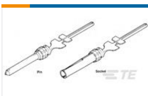
TE Part #5-745288-8 20 DF SKT CONTACT DUPLEX/LP
