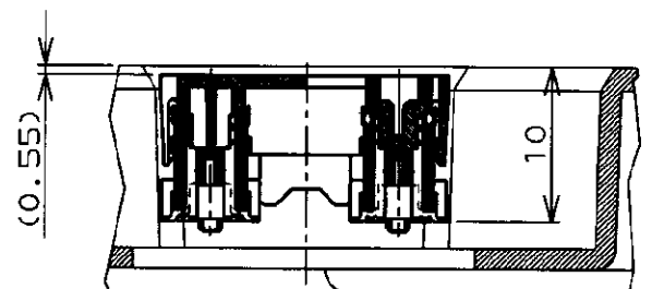
SECT. "B"- "B" (SCALE 2-1)
