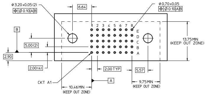
RECOMMENDED PCB LAYOUT AND KEEP OUT ZONE
