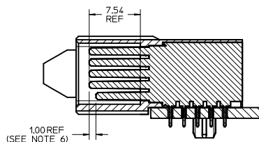
SECTION Z-Z
