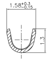
SECTION Y-Y
