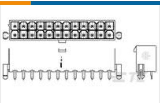
TE Part #1586039-2 2P VAL-U-LOK VRT HDR W/P V2
