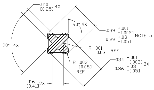
SECTION A-A SCALE NTS ALL DIM TYP WITHOUT FERRULE
