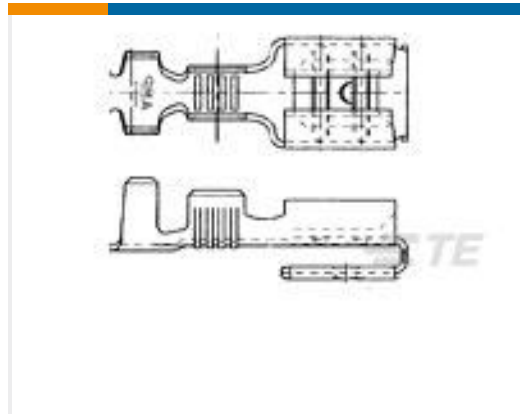
TE Part #160739-1 250 FASTON,PIGGYBACK REC.,18-14 AWG,BR
