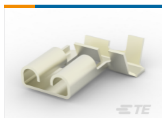
TE Part #2286377-1 250 FASTON,FLAG,REC.,22-18 AWG, NPST
