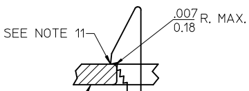
SECTION "E"- "E" NO SCALE
