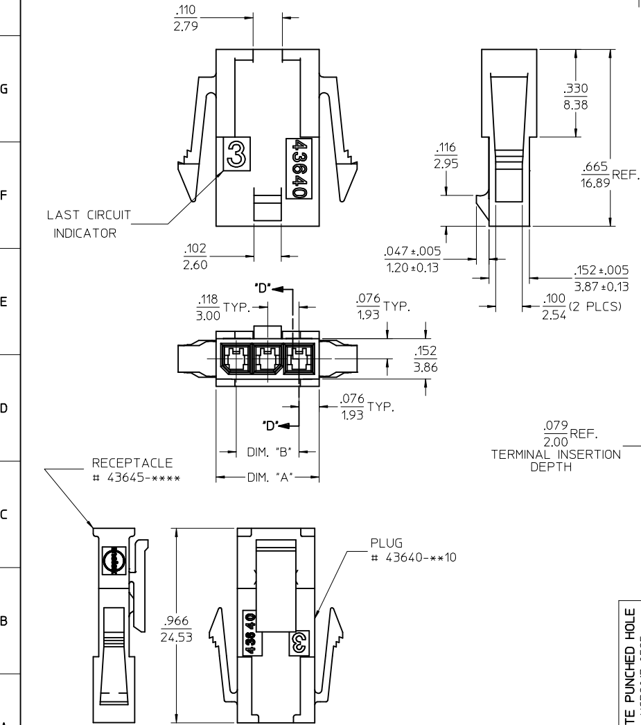
MATED MICRO-FIT CONNECTOR
