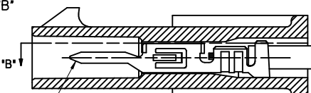
SECTION "D"- "D" WITH TERMINAL NO SCALE
