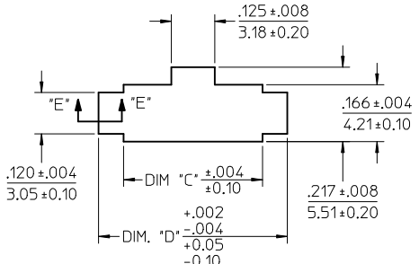
RECOMMENDED PANEL CUT-OUT (SEE NOTES 8 & 11)
