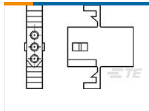
TE Part #770335-1 04P .062 COMM P&S RECPT
