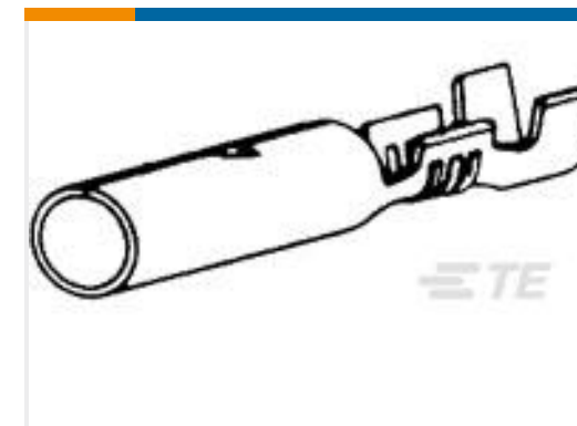
TE Part #60798-4 SHUR PLUG 180 RECEPTACLE 18-14 AWG TPBR
