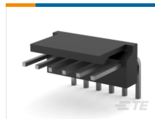
TE Part # 3-647051-6 06P MTA100 HRD ASSYF/L HT LF
