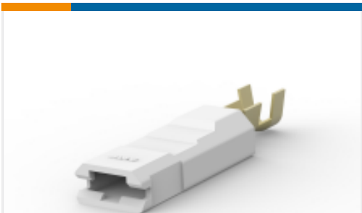
TE Part #1969104-1 ULTRA POD: Straight, Receptacle Assembly, Unplated, .250 inch
