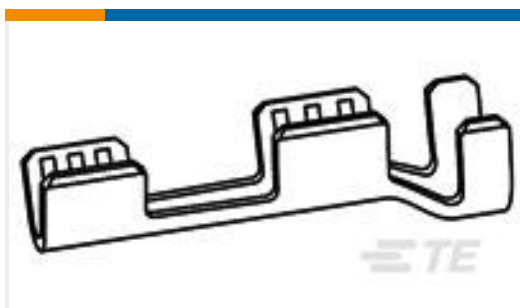
TE Part #62419-3 SPLICE 18-16/18-14 AWG .020 NPST
