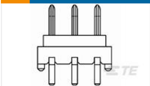
TE Part #6447142-5 BU CONN FS3 HEADER Q2 (6P)
