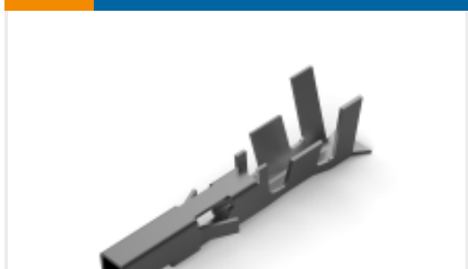
TE Part #1586055-3 VAL-U-LOK SKT PHBZ SN 16AWG
