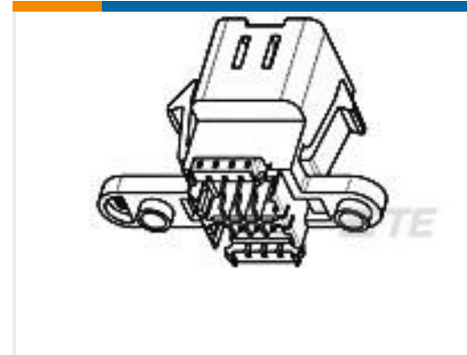
TE Part #176121-2 .040 MULTI-LOCK 8 POS
