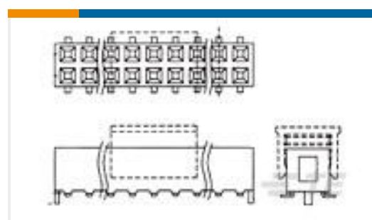
TE Part #2023519-1 ASSY AMPMODU 2MM PLUG SMT-TYPE CONN.
