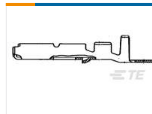
TE Part #172773-2 MIC MK-2 REC B TYPE
