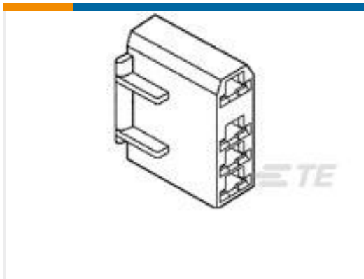
TE Part #520987-1 250 FASTON HSG. REC. 4P BLACK
