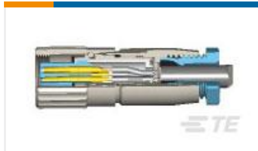
TE Part #3-1437719-0 T01-0550-S03-FEMALE PLUG CONNECTOR SOLDE
