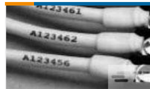
TE Part #505325P099 RNF-100-3/4-A1-RD-30MM
