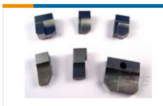
TE Part #2-1803001-1 ANVIL,COMBINATION, END FEED
