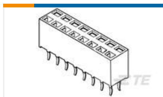
TE Part #215309-4 2X4P HV100 REC CON. TE, 8.5MM
