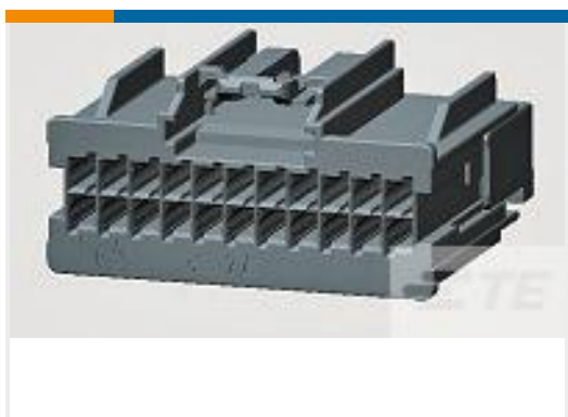
TE Part #2208021-2 22POS,0.64 GENER. Y,REC HSG,ASSY
