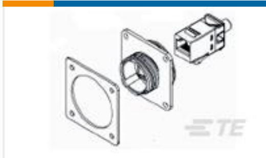
TE Part #1546908-1 CPC RCP ASSY, IND ETHERNET, SHLD
