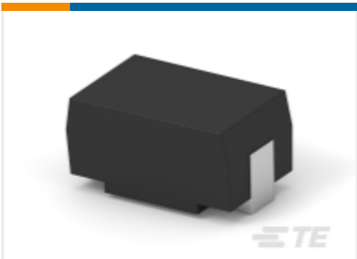
TE Part #3-1879233-3 SMD Power Resistor: 7 Watt, 200-2M Ohm
