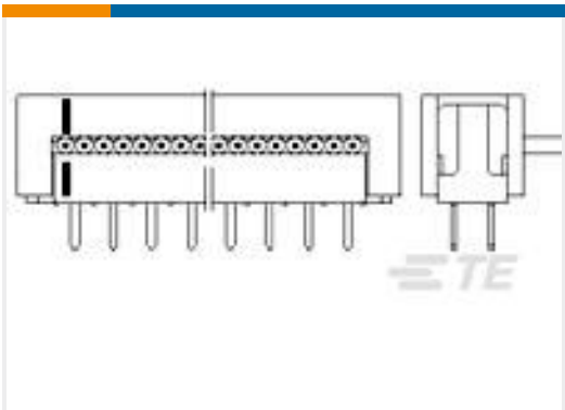
TE Part #1-216093-0 AMP-LATCH PRE-ASSY DIL WITHO
