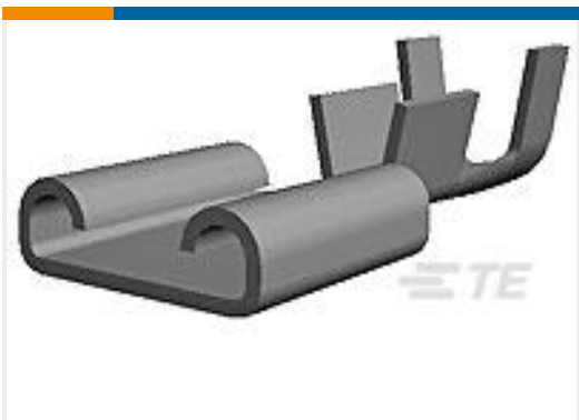
TE Part #1-160304-2 250 FASTON, REC., 14-17AWG, TPBR
