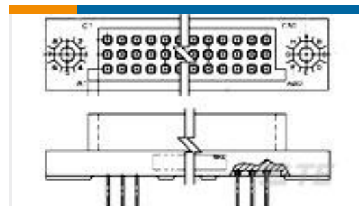
TE Part #447208-1 3 ROW BOX RECP 240 POS 100 C/L
