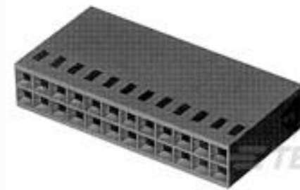
TE Part # 1-87456-5 20 MODIV HSG COMP DR .100CL
