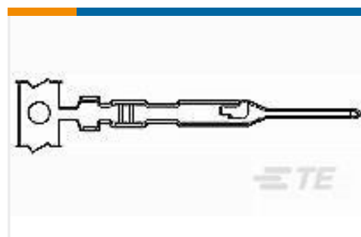
TE Part #5-104505-4 MTE PIN 22-26 AWG PLTD
