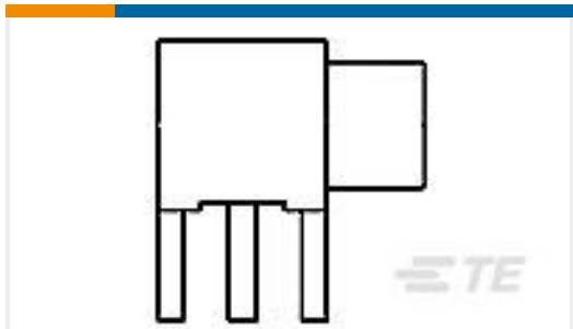
TE Part #1061027-1 5864 5002 10,OSX RA PCB JACK
