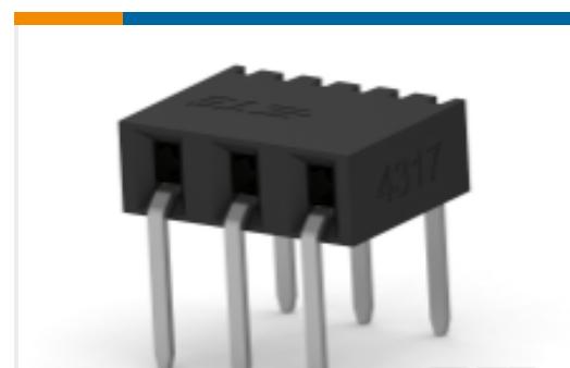
TE Part #2314936-3 3P,2MM,B-B,REC,SRHZ,2.8,0.1AU,TR
