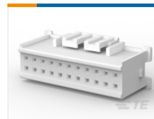
TE Part # 2-1969540-2 HOUSING, PLUG, 22P,DUAL ROW, EP2.5
