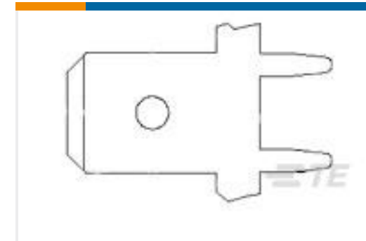
TE Part #1217539-1 250 FASTON, PCB TAB, TCBR
